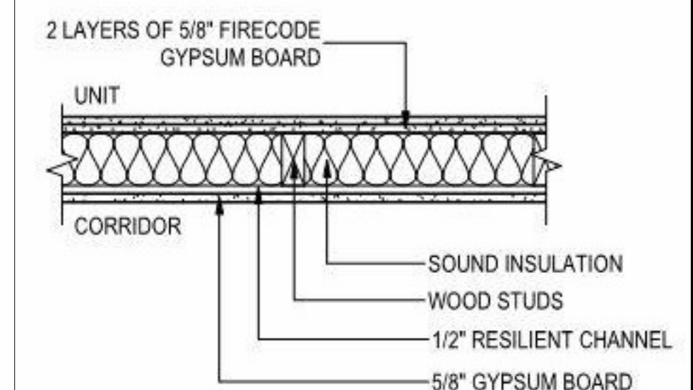
1 HOUR RATED WALL UL DESIGN U311 STC 50 - 54
