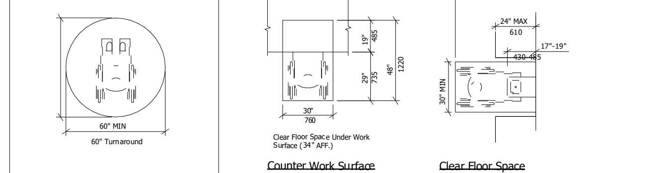
TURNING RADIUS WORK COUNTER
