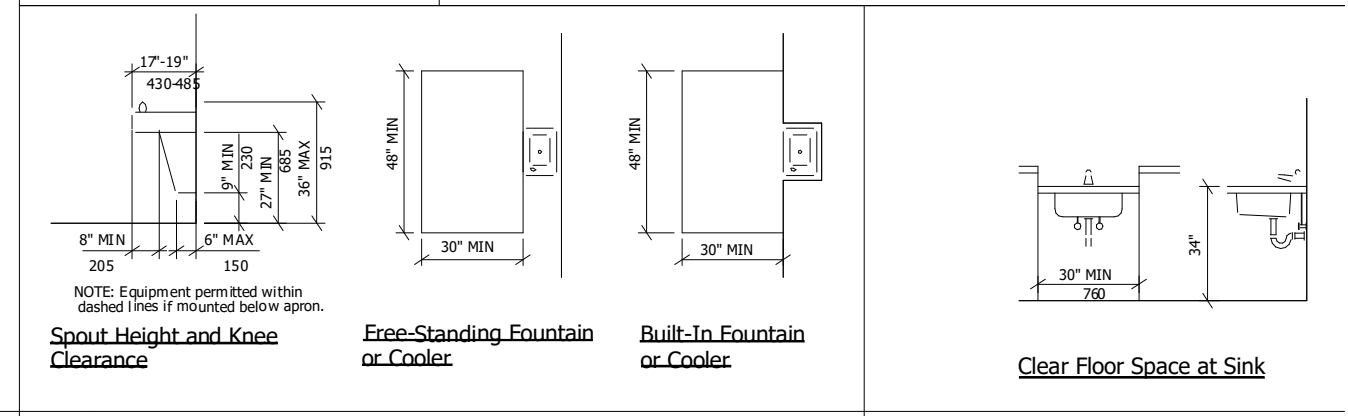
DRINKING FOUNTAIN / WATER COOLER SINK
