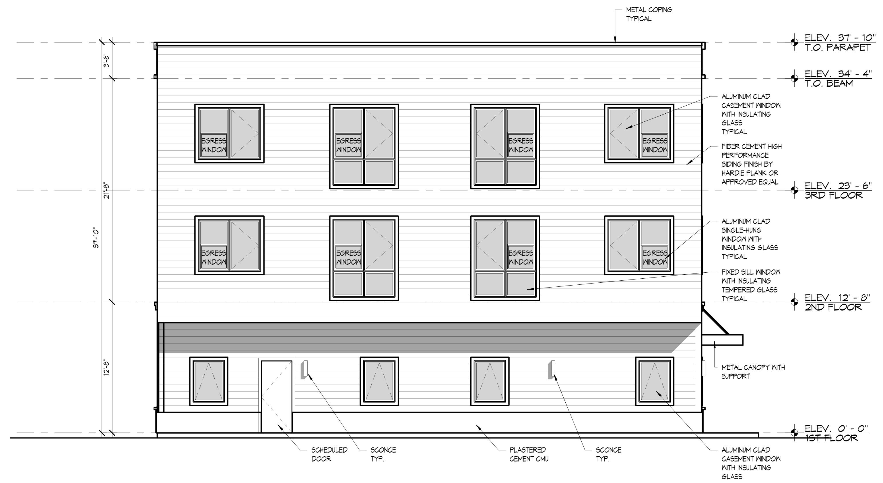
2 NORTH ELEVATION 3/16" = 1'-0"
