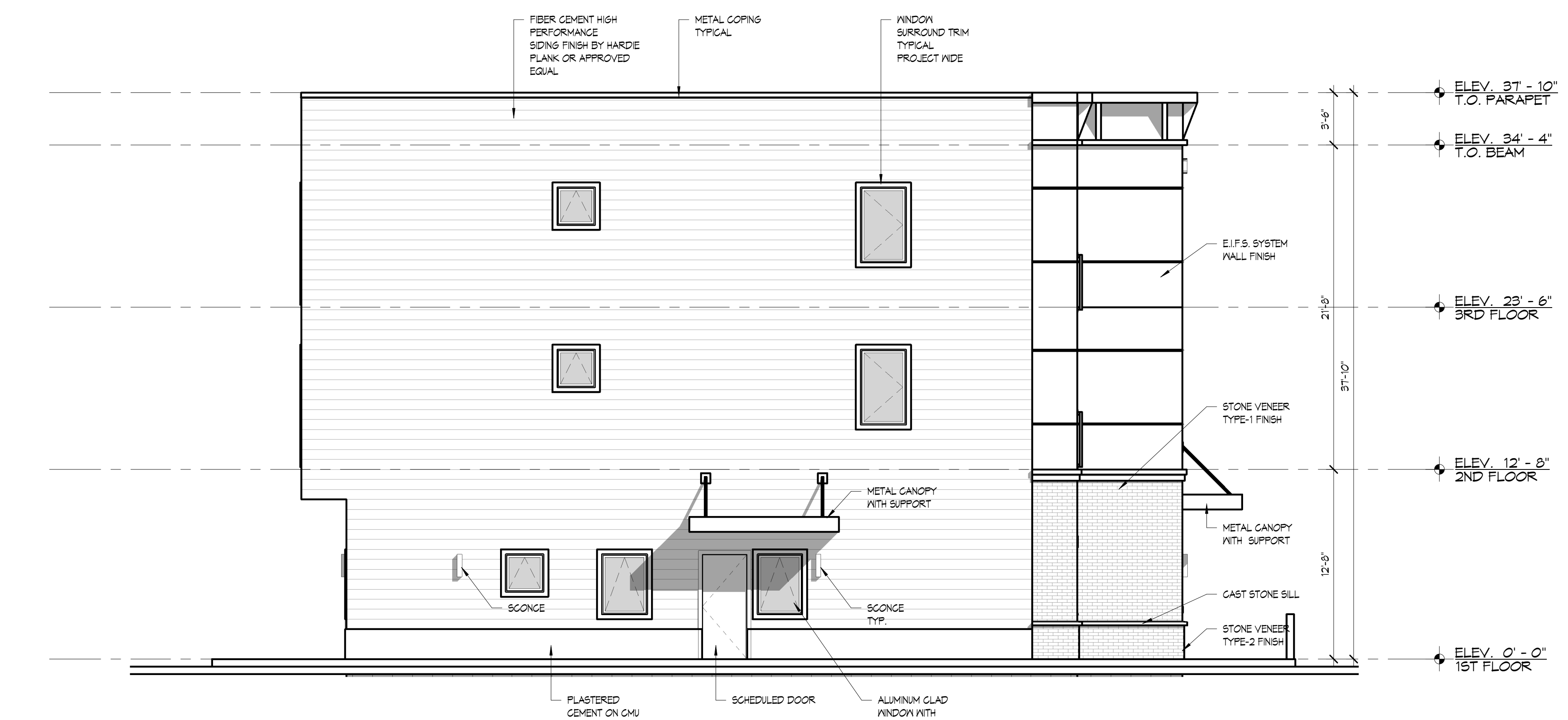
2 WEST ELEVATION 3/16" = 1'-0"
