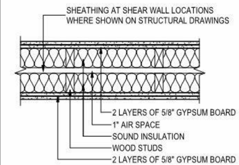
1 HOUR RATED WALL UL DESIGN - U341 STC 63 MIN.
