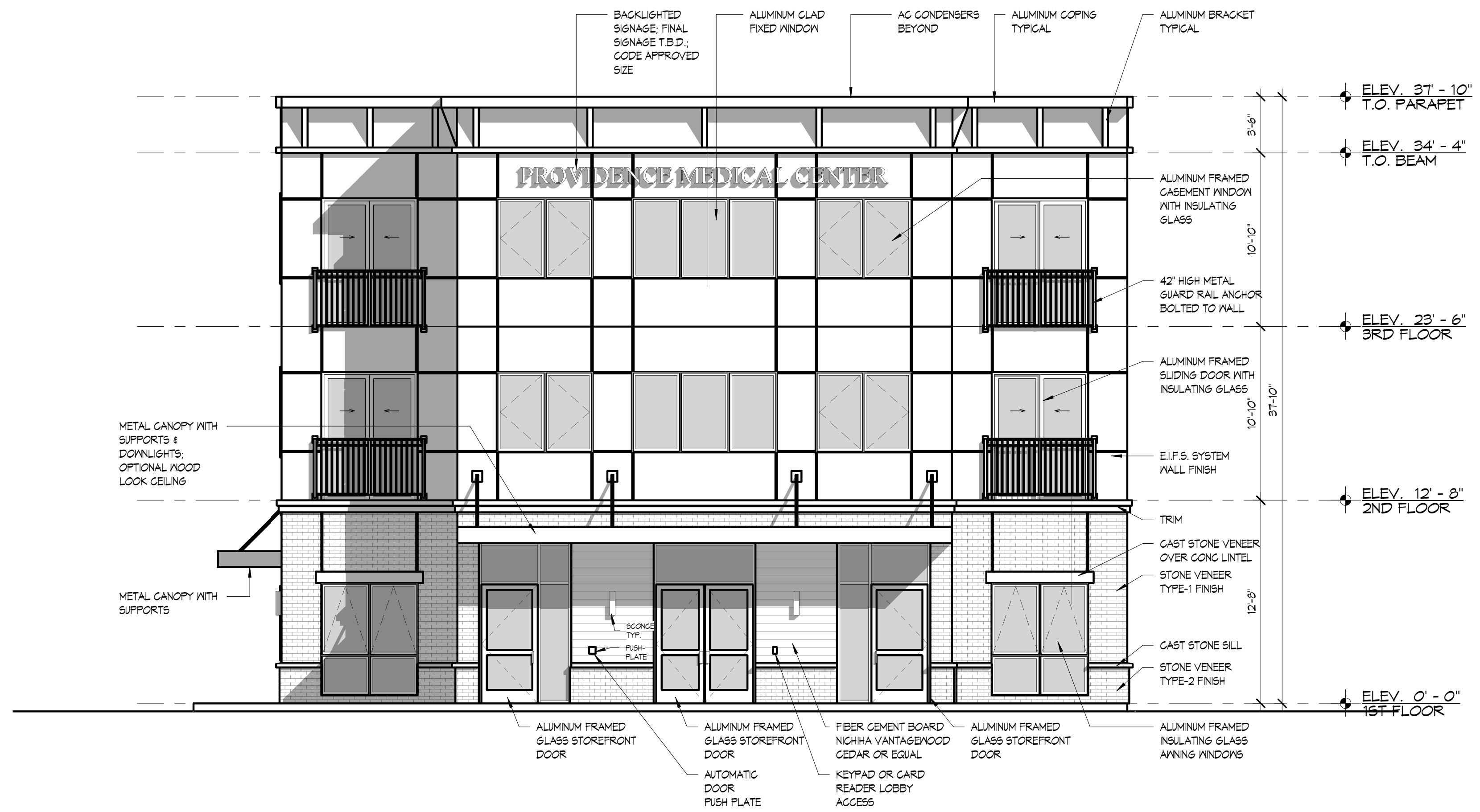
1 SOUTH ELEVATION 3/16" = 1'-0"
